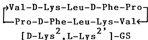
Fig. 1. Primary structure of gramicidin S and its analogs.
